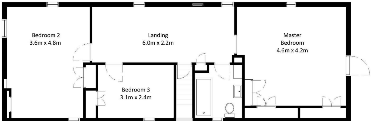
Clos de Dixcart First Floor Plan
